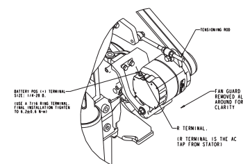
DETAIL OF BATTERY CHARGING ALTERNATOR CONNECTIONS SCALE 1:3
