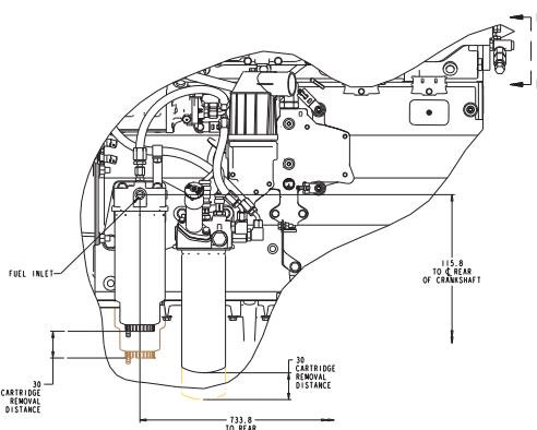
DETAIL OF FUEL FILTER HEAD ASM SCALE 1:2
