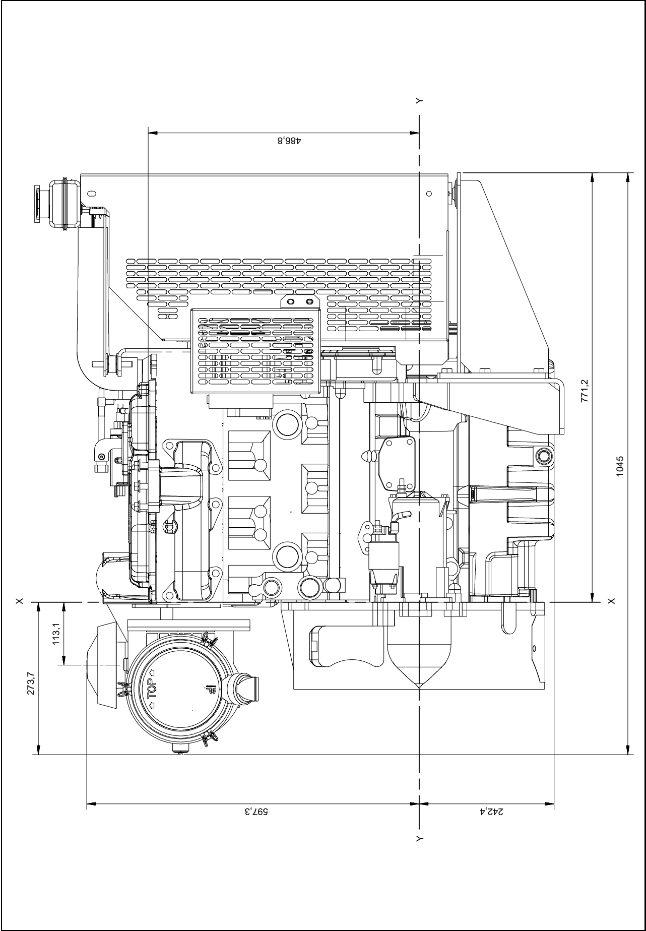
1103C-33 G2 ElectropaK - right side view
